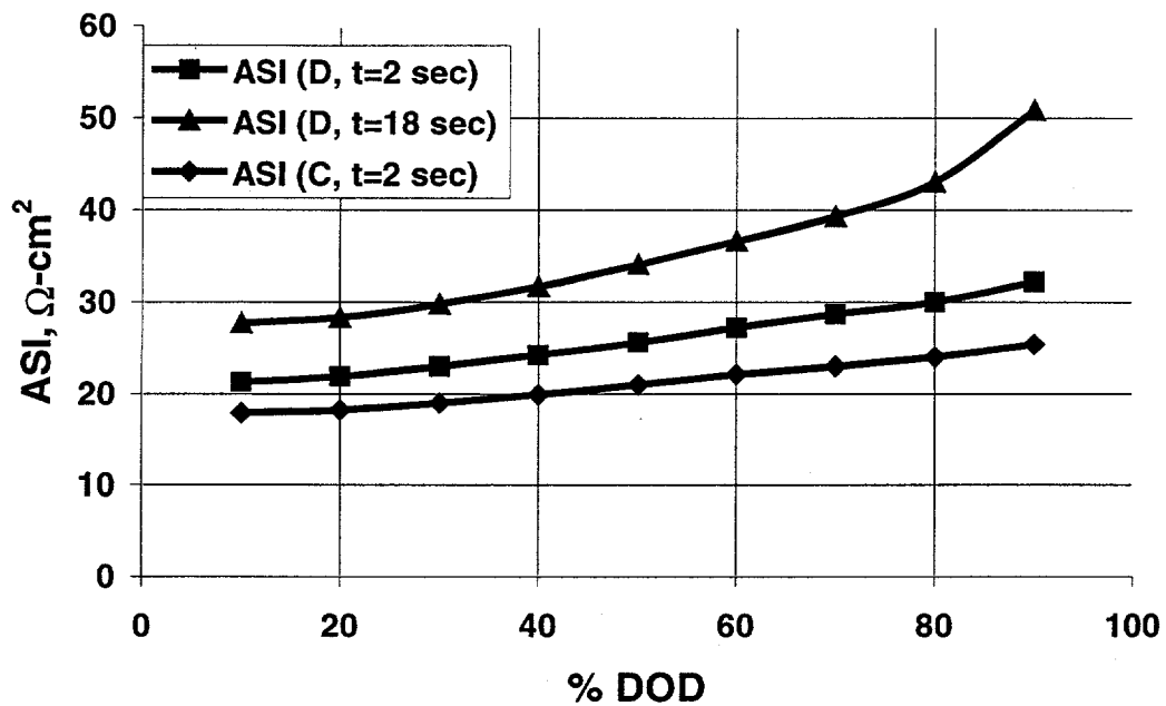
Fig. 5. Pulse-power area specific impedance (ASI) for a \text{Li}_4\text{Ti}_5\text{O}_{12}/\text{LiCoO}_2 cell obtained after 47,500 cycles of the PNGV 100-Wh Test Profile.
