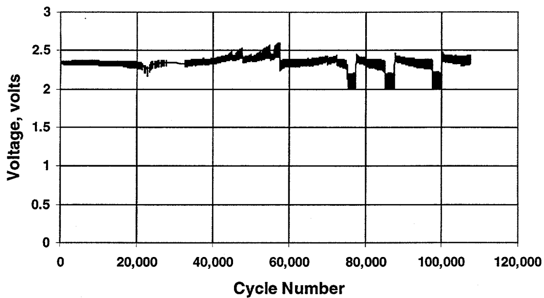
Fig. 3. Voltage profile for a \text{Li}_4\text{Ti}_5\text{O}_{12}/\text{LiCoO}_2 cell operated under the PNGV 100-Wh Test Profile. Data shown for every 200 th cycle.
