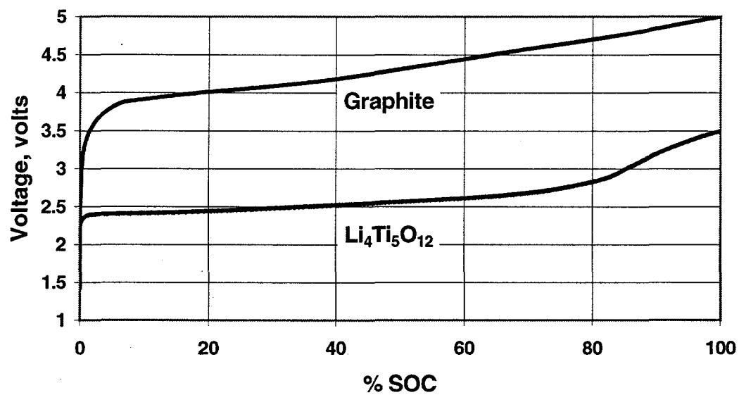
Fig. 1. Inherent safety provided by the rise in voltage at the end-of-charge for the \text{Li}_4\text{Ti}_5\text{O}_{12}/\text{LiCoO}_2 cell couple. No such end-of-charge indicator exists for the graphite/ \text{LiCoO}_2 couple.
